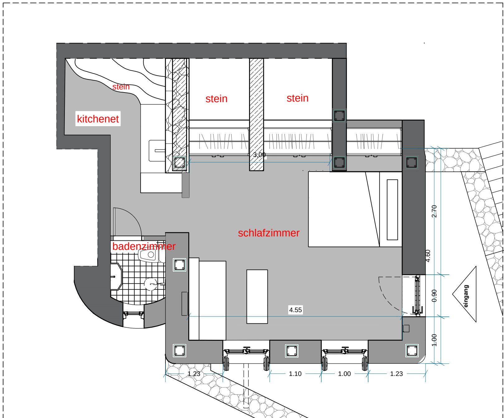
Alkyon Villas-Villa K5,ebene 0
